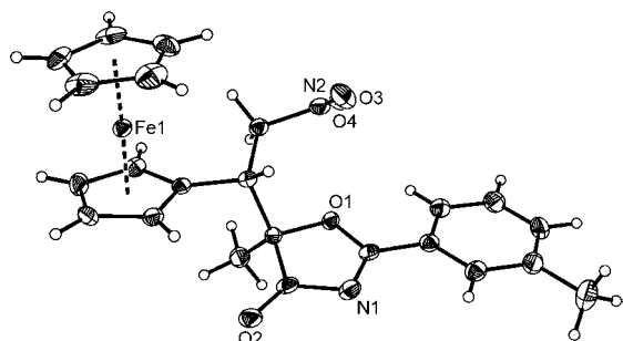
Figure 1. Single crystal X-ray diffraction analysis of 27 . Thermal ellipsoids at 50% probability.
