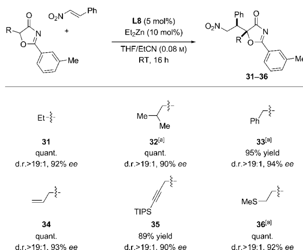
Scheme 4. Scope of 5-alkyloxazole-4(5 H )-ones. All reactions were run on a 0.125 mmol scale under the conditions described in Scheme 1 with L8 (0.08 M) in propionitrile. Yields of isolated products are given. The diastereomeric ratios were determined by ^1\text{H} NMR analysis of the crude mixture. The ee values were determined by HPLC analysis. [a] \beta -nitrostyrene:oxazolone 1:1 (0.1375 mmol).
