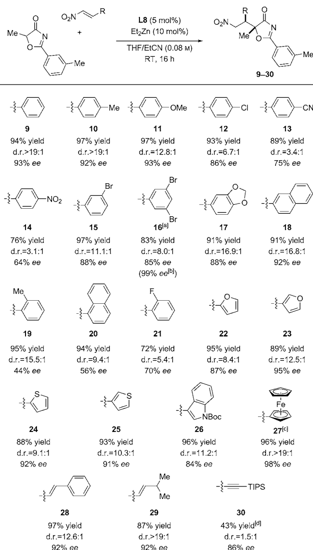
Scheme 3. Addition of 5-methyloxazole-4(5H)-one to various nitro olefins. All reactions were run on a 0.125 mmol scale under the conditions described in Scheme 1 with L8 (0.08 M) in propionitrile. Yields of isolated products are given. The diastereomeric ratios were determined by 1 H NMR analysis of the crude mixture. The ee values were determined by HPLC analysis. [a] 0.5 mmol scale; reaction on a 0.125 mmol scale: 90% yield, d.r. = 8.4:1, 84% ee . [b] From the mother liquor of a single recrystallization. [c] Absolute configuration established as ( R,R ) by single crystal X-ray analysis. [d] Yield of the major isomer.
