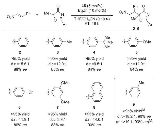
Scheme 2. Optimization of the nucleophile structure. All reactions were run on a 0.125 mmol scale under the conditions described in Scheme 1 with L8 and different nucleophiles. Yields were determined by 1 H NMR spectroscopy with mesitylene as internal standard. The diastereomeric ratios were determined by 1 H NMR analysis of the crude mixture. The ee values were determined by HPLC analysis. [a] Reaction conducted in propionitrile (0.08 M).
